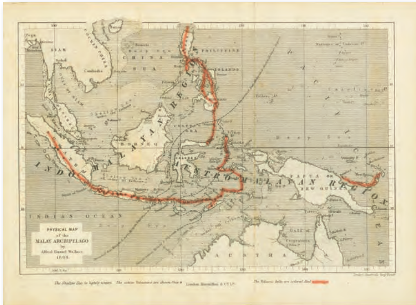
Physical map of the Malay Archipelago by Alfred Russel Wallace, 1868. From no. 766, SCR fDS601 W18
