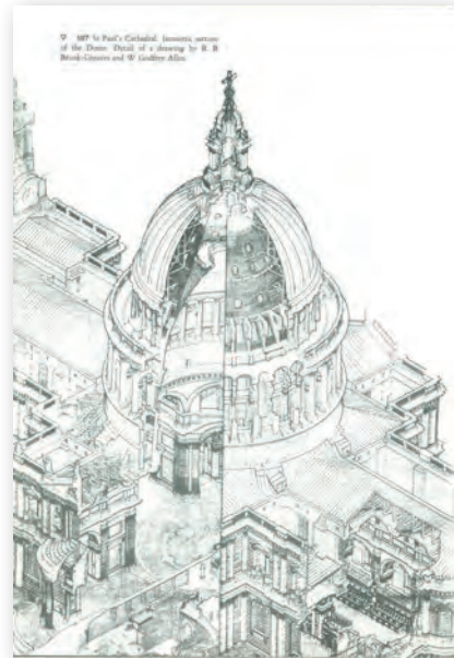
St Paul's Cathedral. Isometric section of the Dome. Detail of a drawing by R.B. Brook-Greaves and W Godfrey Allen; Sir Christopher Wren, Portrait, c. 1683 by Johann Baptist Closterman. From no. 108, NA997 W94
